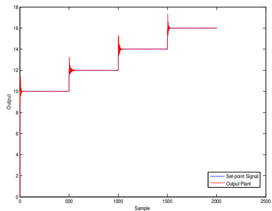
Fig.7. Time response characteristic of control systems with GA-FWNN (Test process)
