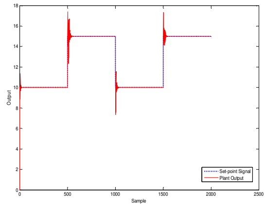
Fig.6. Time response characteristic of control systems with GA-FWNN (Learning process)
